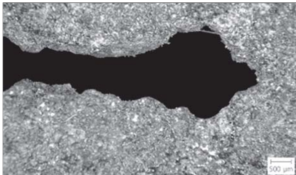
Obr. 2 diera - detail
